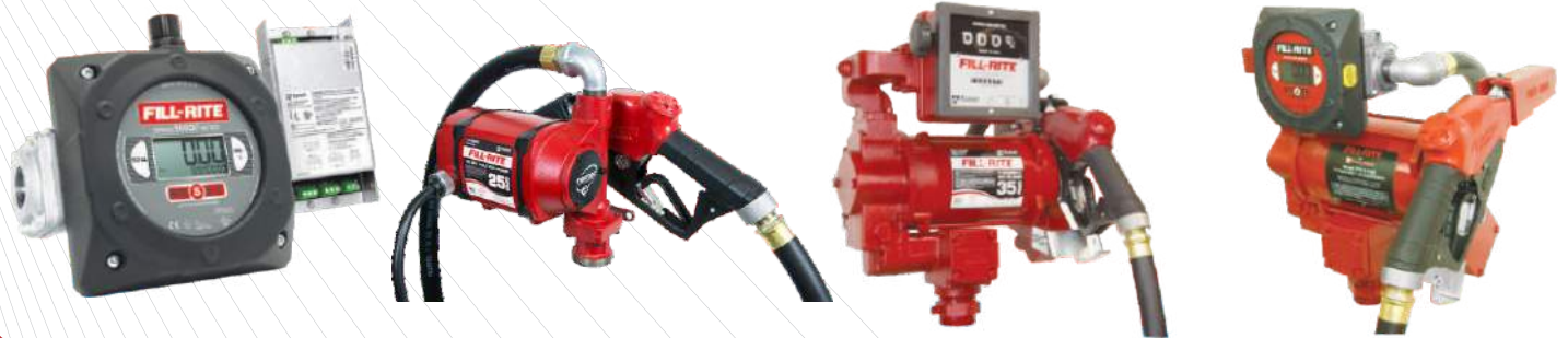
High Flow AC & DC Pumps, Air Operated Diaphragm Pumps & Meters (Mechanical & Electronic) with Hose & Nozzle
