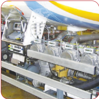
Sealed Delivery Systems
